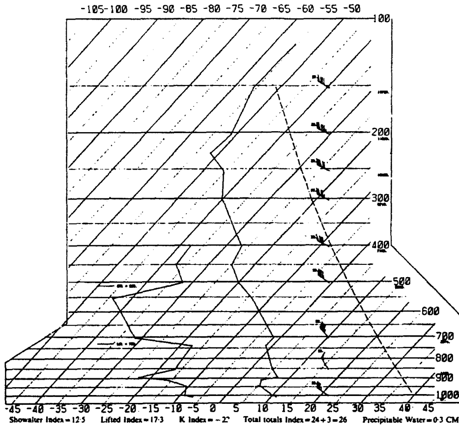
Figure 9. Radiosonde profile showing temperature and dew point in ^{\circ}\text{C} for Kodiak, Alaska, 00.00 UTC, 24 September 1986. Wind barbs show speed in knots: 1 barb = 10 kts ( 5\text{ m s}^{-1} ); \frac{1}{2} barb = 5 kts ( 2\frac{1}{2}\text{ m s}^{-1} ); a pennant = 50 kts ( 25\text{ m s}^{-1} ).
